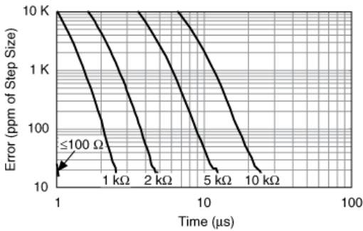
NI 6255 Settling Error Versus Time for Different Source Impedances
