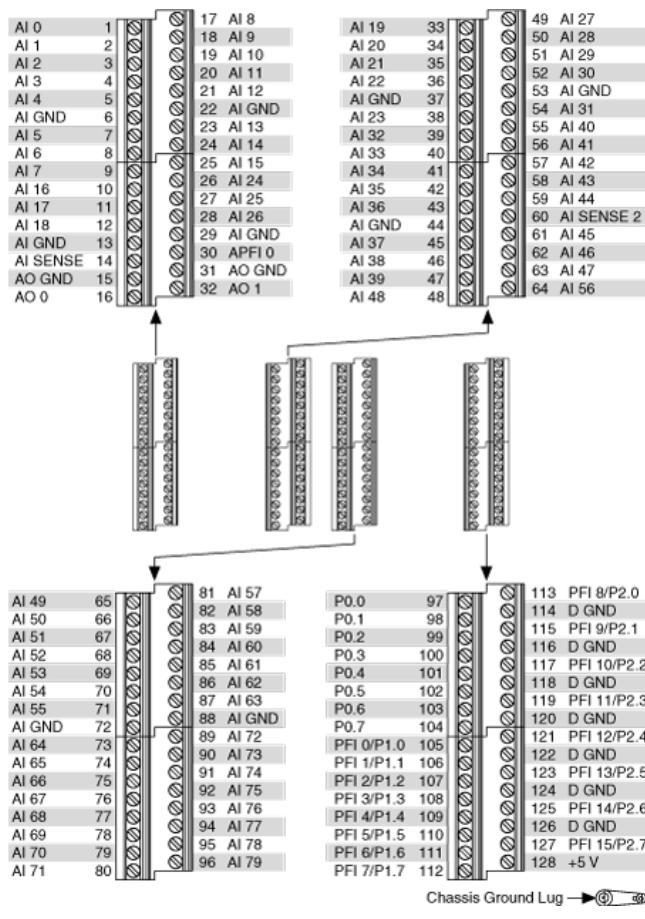
NI USB-6255 Screw Terminal Pinout
