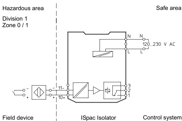
Connection diagram 9170/11-12-21
